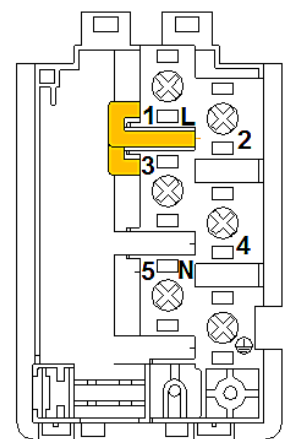
Heater de-rated to 6.75kW
