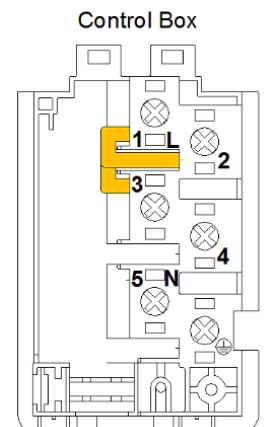
Air Curtain de-rated to 2kW
